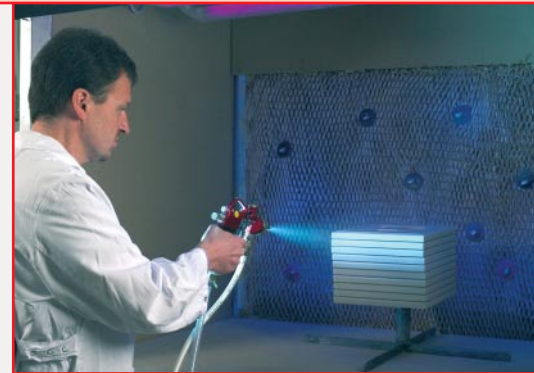
Processing of DORUS® 3D adhesives
